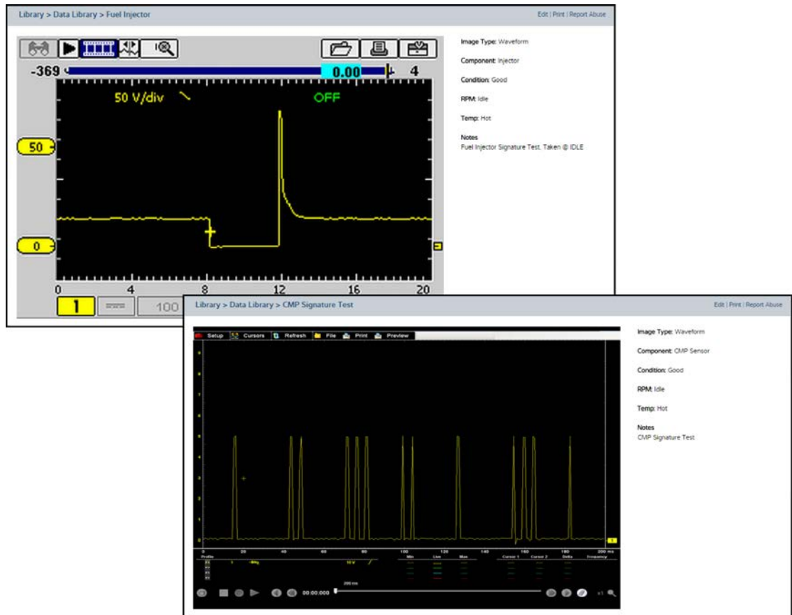
Figure 9-41 SureTrack - Waveform examples
