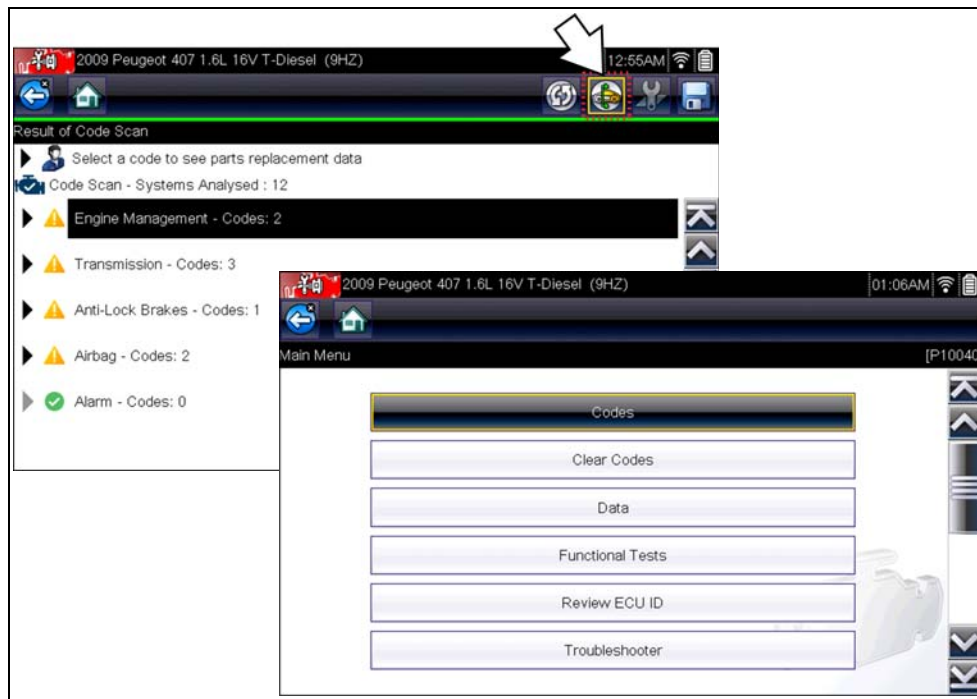
Figure 4-5 System icon (opens Main Menu)
