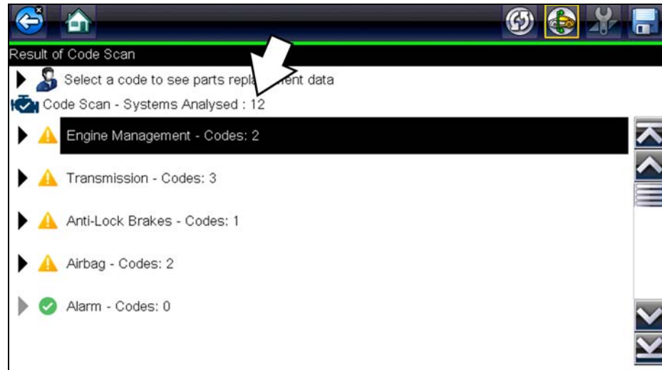
Figure 4-4 Code Scan systems analyzed result total
