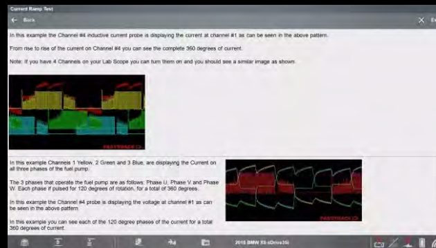
Full-color waveform display for the 3-phase brushless fuel pump system on a 2018 BMW X6 sDrive35i.
